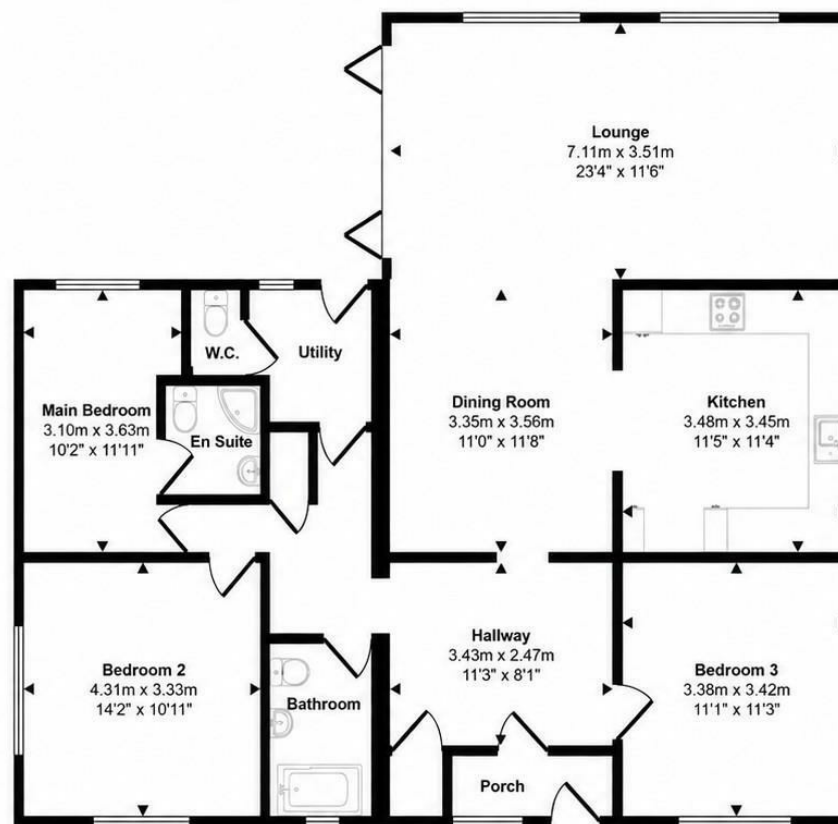
Floorplan Approx 122 sq m / 1311 sq ft
